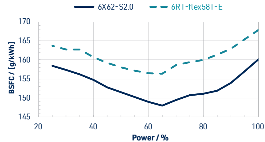
Comparison: Specific fuel consumption between 6RT-flex58T-E and 6X62-S2.0 rated at 12 900 kW / 105 rpm
